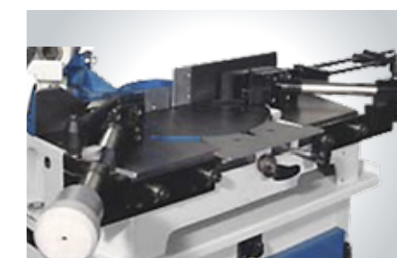
Double horizontal clamps: 45° mechanical with foot-pedal 45° pneumatic with foot-pedal 90° pneumatic with lever
